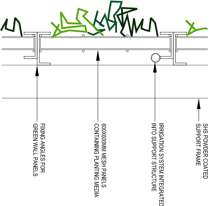
INDICATIVE DETAIL OF GREEN WALL PANELS
